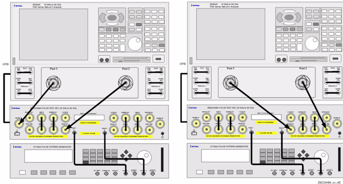
Figure 46 On/Off Switch Ratio
