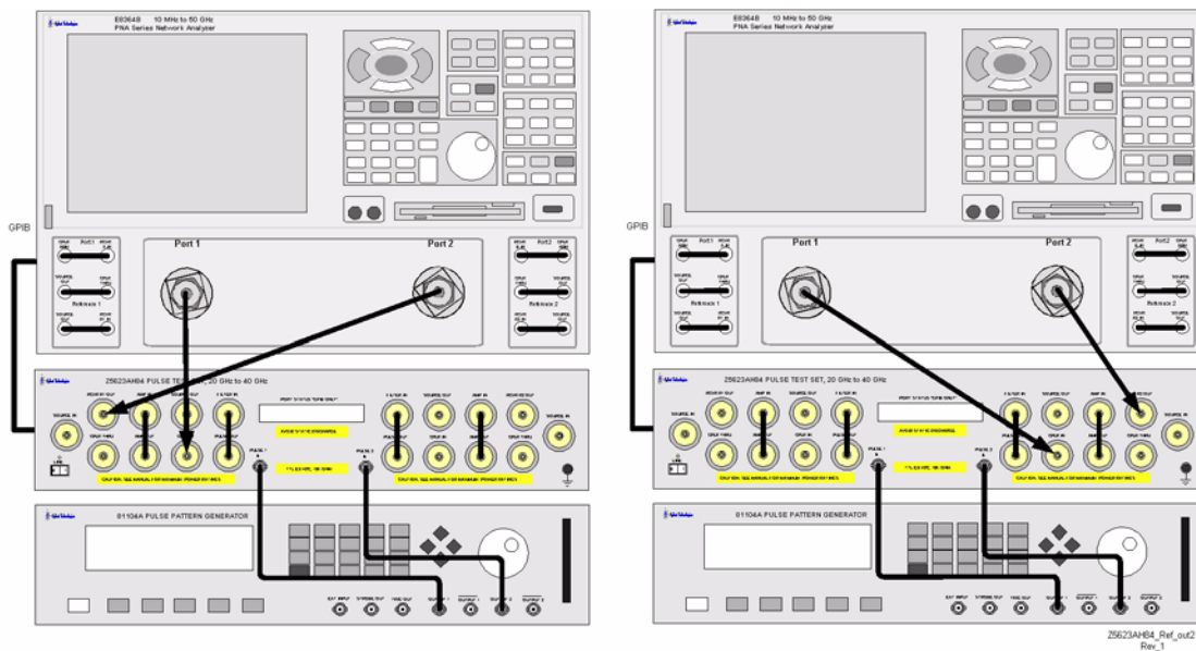
Figure 47 Attenuator Steps
