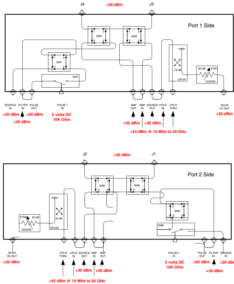
Figure 11 Shipped Configuration
