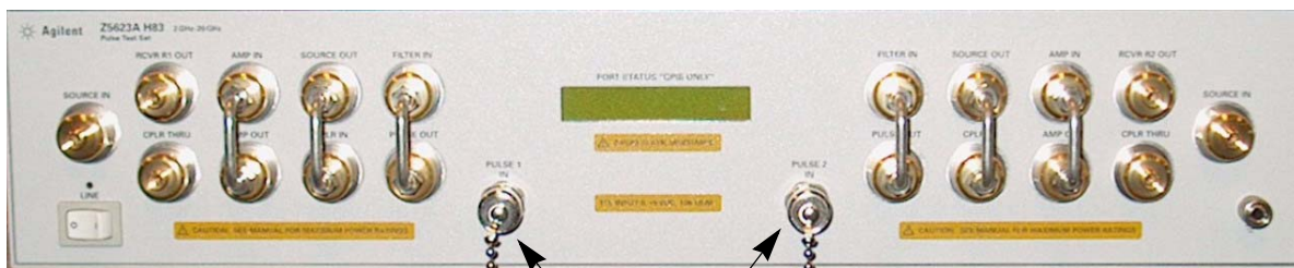
Figure 11 Shipped Configuration
