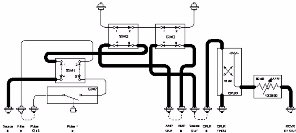
Figure 40 High Power
