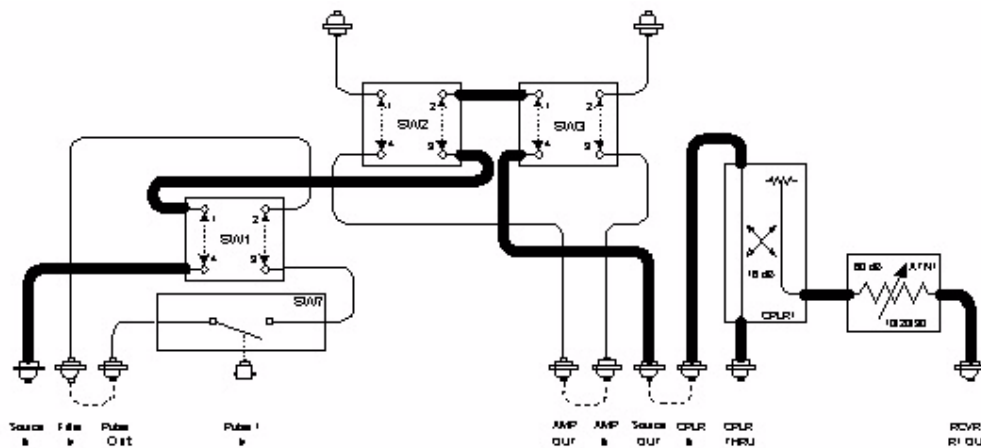
Figure 39 Bypass
