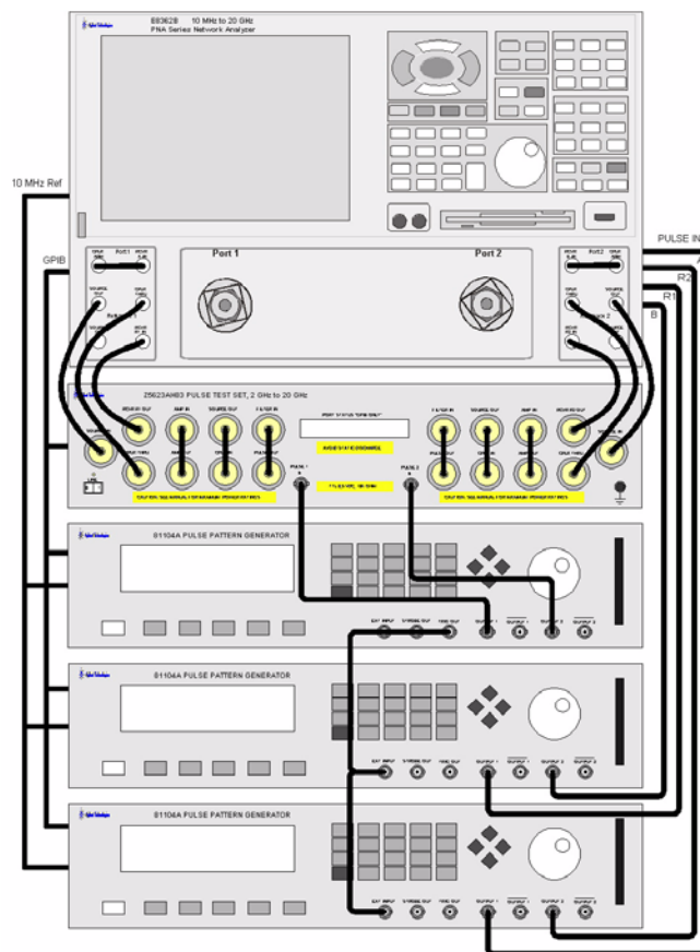
Figure 35 Setup Configuration
