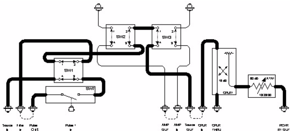
Figure 41 Pulse
