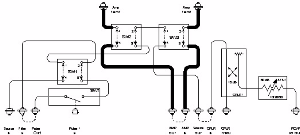
Figure 43 Amplifier Termination
